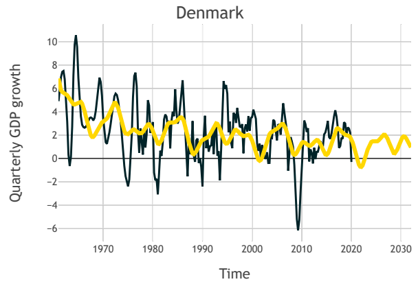
Figure 6: harmonic regression fit for Denmark.
