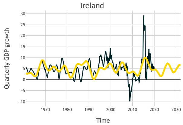
Figure 12: harmonic regression fit for Ireland.
