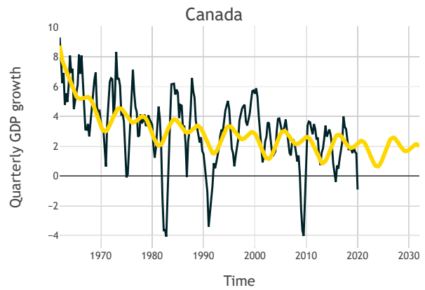
Figure 4: harmonic regression fit for Canada.
