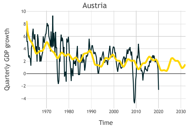
Figure 2: harmonic regression fit for Austria.
