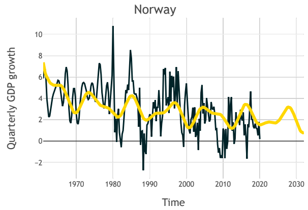
Figure 18: harmonic regression fit for Norway.
