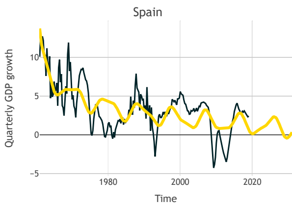
Figure 21: harmonic regression fit for Spain.
