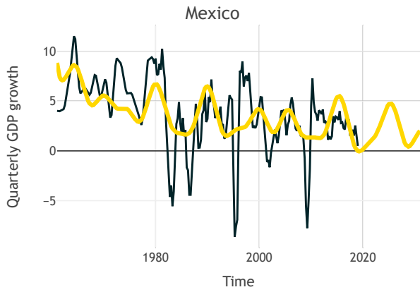
Figure 17: harmonic regression fit for Mexico.
