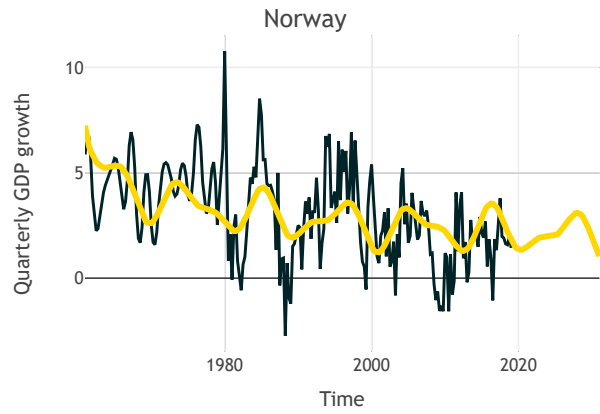
Figure 18: harmonic regression fit for Norway.
