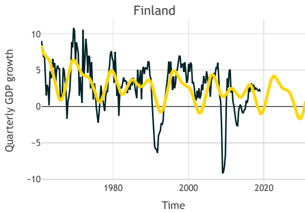
Figure 7: harmonic regression fit for Finland.
