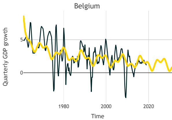
Figure 3: harmonic regression fit for Belgium.
