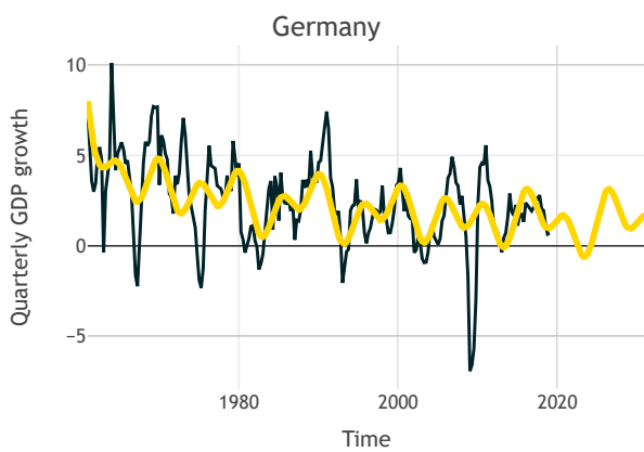
Figure 9: harmonic regression fit for Germany.
