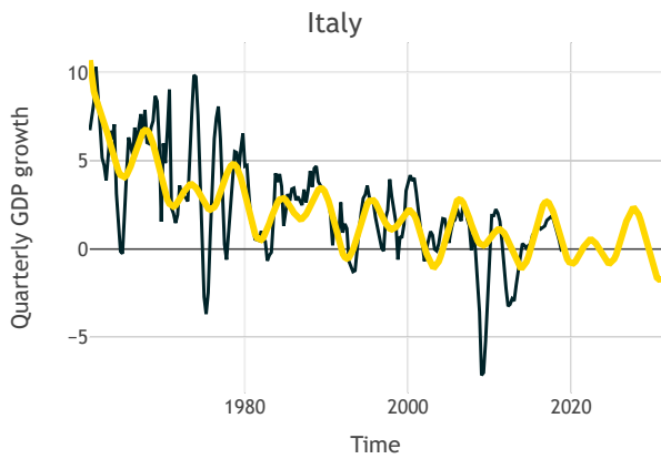
Figure 13: harmonic regression fit for Italy.
