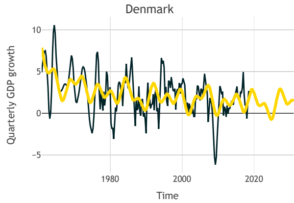
Figure 6: harmonic regression fit for Denmark.
