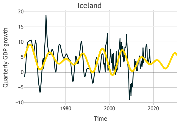
Figure 11: harmonic regression fit for Iceland.
