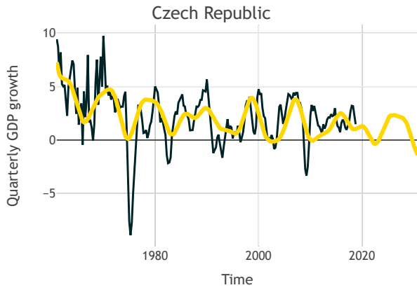
Figure 5: harmonic regression fit for Czech Republic.
