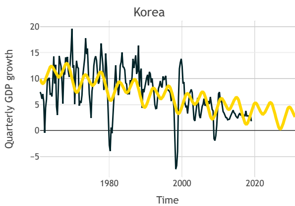
Figure 15: harmonic regression fit for Korea.
