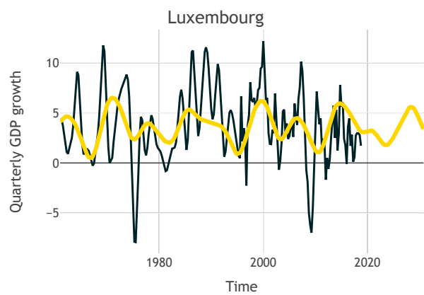
Figure 16: harmonic regression fit for Luxembourg.
