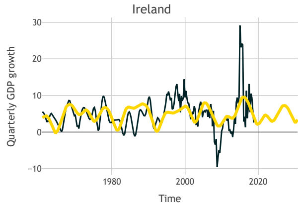
Figure 12: harmonic regression fit for Ireland.
