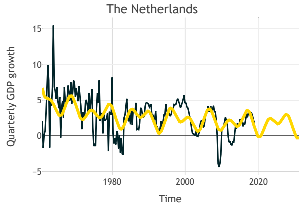
Figure 24: harmonic regression fit for The Netherlands.
