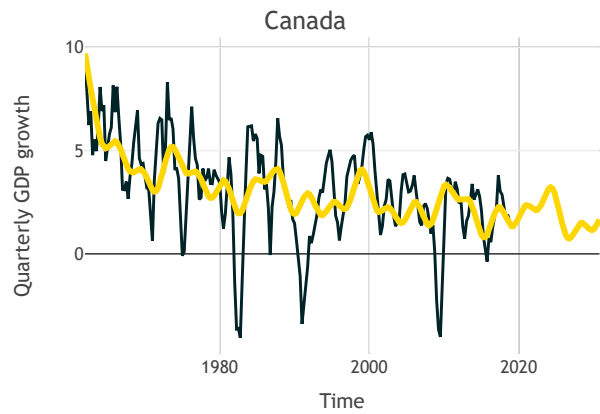
Figure 4: harmonic regression fit for Canada.
