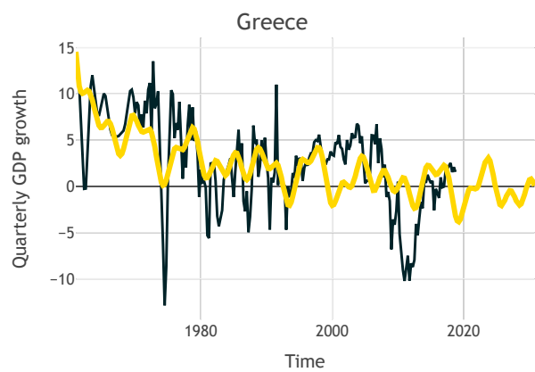
Figure 10: harmonic regression fit for Greece.
