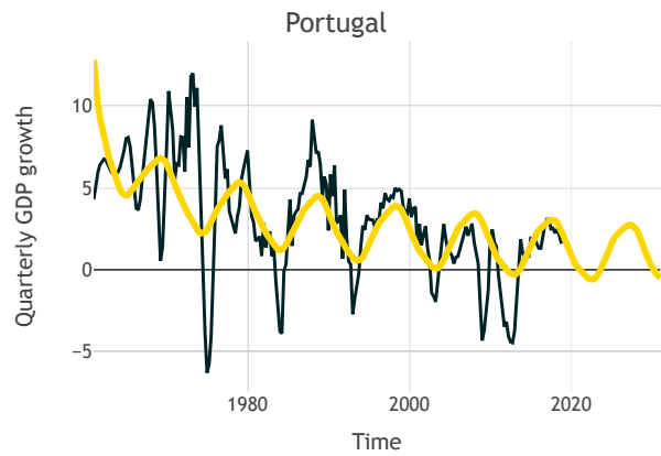
Figure 20: harmonic regression fit for Portugal.
