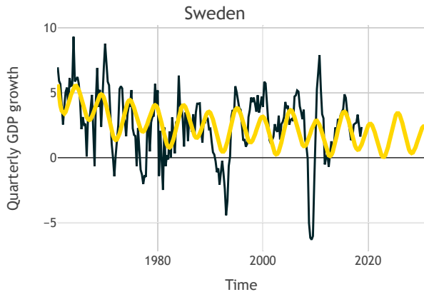
Figure 23: harmonic regression fit for Sweden.
