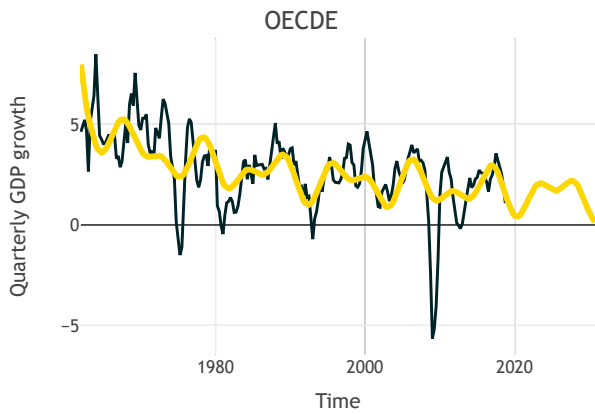
Figure 19: harmonic regression fit for the European OECD countries.
