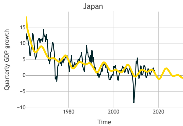
Figure 14: harmonic regression fit for Japan.
