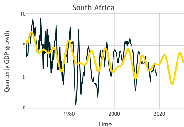
Figure 22: harmonic regression fit for South Africa.
