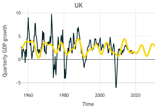
Figure 25: harmonic regression fit for UK.
