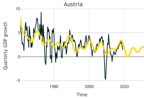
Figure 2: harmonic regression fit for Austria.
