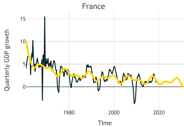
Figure 8: harmonic regression fit for France.
