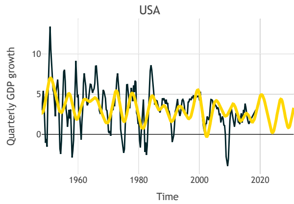
Figure 26: harmonic regression fit for USA.
