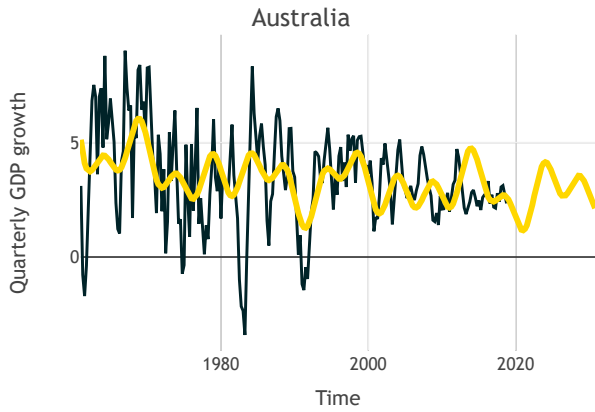
Figure 1: harmonic regression fit for Australia.
