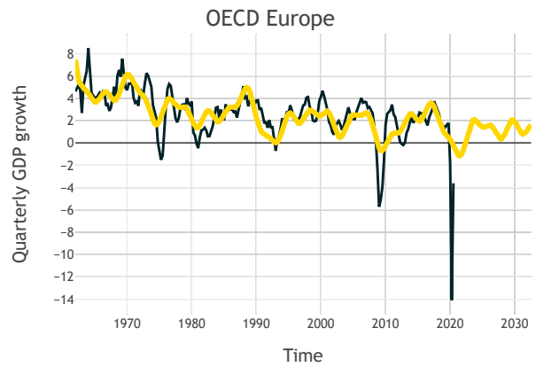
Figure 20: harmonic regression fit for the European OECD countries.
